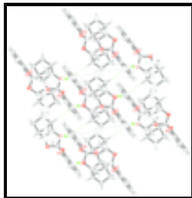
Fig. 2. The crystal packing viewed along [0 1 0]. Green arrows: the strongest C—H \cdots O interaction in terms of the H \cdots O distance (C14—H14 \cdots O2). Green dotted lines: the strongest C—H \cdots \pi interaction (C5—H5—C _g , C _g is the centroid of the phenylene residue).
